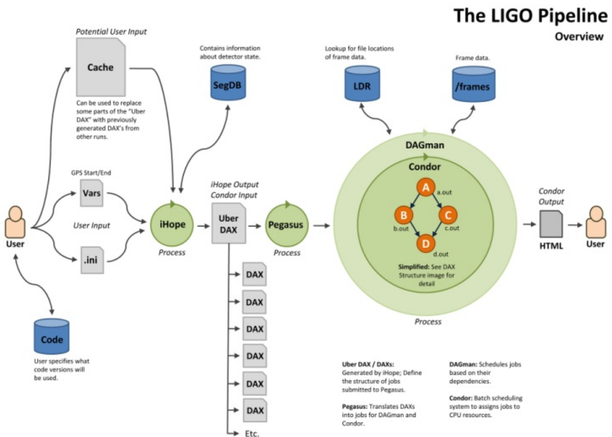
Figure 4. The final LIGO pipeline overview visualization.
